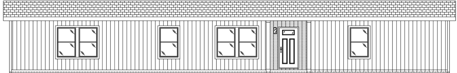
FRONT SIDEWALL
